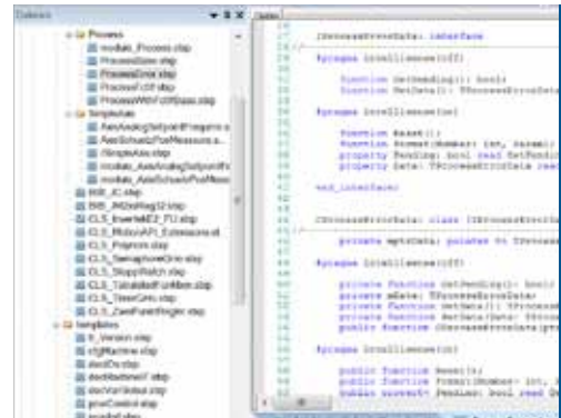
Pragma INTELLISENSE(OFF)
